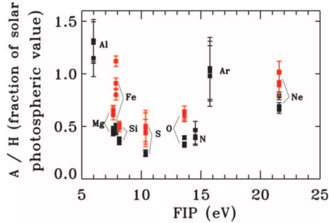
Fig. 19 Abundances relative to hydrogen vs. the first ionization potential (FIP) in quiescent (black) and flaring (red) intervals in Chandra spectra of the RS CVn \sigma^2 Coronae Borealis. Figure reproduced from Osten et al (2003) with permission. They note that there is a slight enhancement of Mg, Si, O, and Ne during the flare, and Fe increases by nearly twice.
