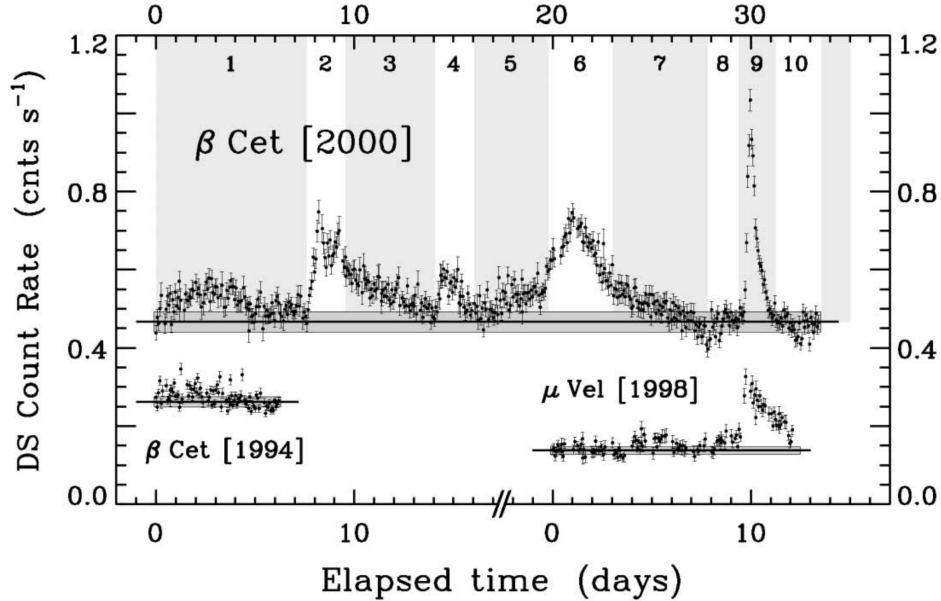
Fig. 6 A small fraction of single, red clump giant stars like \beta Ceti exhibit continuous variability that consists of week-long, giant EUV ( 60 - 180 \text{ \AA} ) flares. A flare on \mu Velorum (also shown) is even more unexpected in its evolutionary stage. Figure reproduced from Ayres et al (2001) with permission.
