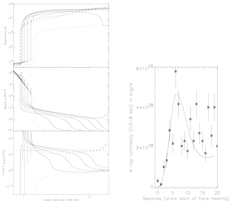
Fig. 23 ( Left ) Hydrodynamic modeling of a coronal explosion on CN Leo. The panel shows temperature, number density, and the emission measure weighted cooling function. The solid lines show the evolution at t = 0, 2, 4, 8, 10 s when a flare heating function was applied, while the dashed lines correspond to t = 13, 16, and 19 s. ( Right ) Modeled X-ray light curve over the first 20 s of the model compared to XMM-Newton data of the early phase of the giant X-ray flare. Figures reproduced from Schmitt et al (2008) with permission.
