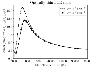
Fig. C6 Balmer jump ratios calculated from the LTE emissivity models in Fig. C5 and from the same calculations of the LTE emissivity in a hydrogen gas with a density of \rho = 10^{-9} \text{ g cm}^{-3} .
