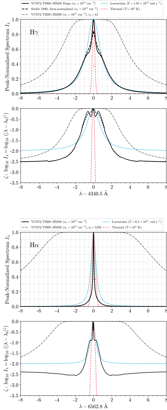
Fig. 25 Optically thin spectral line profiles from the TB09+HM88 pressure broadening theory for Balmer H \gamma (top two panels) and H \alpha (bottom two panels) at n_e \approx 10^{15} \text{ cm}^{-3} . These are identical to the Vidal et al (1973) (VCS73) calculations at this density, and they do not include thermal Doppler convolution in this figure. The 2nd and 4th panels show the slopes, \eta , calculated for each of the profiles in 1st and 3rd panels. Lorentzian profiles with scaled damping widths are overplotted for comparison. The slope of the H \alpha pressure broadening profile is between the Holstmark and Lorentzian because of the higher importance of collisional broadening from electrons for this transition. The higher order lines, including H \gamma , are more obviously dominated by the quasistatic (Holtsmark-distributed) perturbations ( cf. Fig 3 of Vidal et al, 1971), are less optically thick, are closer to LTE because of less scattering in this line, and are less affected by thermal broadening (the FWHM of H \alpha is affected by thermal Doppler broadening even at such high densities; 1/e Doppler widths are indicated by horizontal red lines). The “self-broadening” of hydrogen is relatively less in H \gamma and in the higher order lines, but it is important when the atmosphere is largely neutral (Barklem et al, 2000). The Balmer H \gamma line is also less affected by thermal, T = 10^4 K ion-dynamic effects Stehle (1994): we show an area-normalized (rather than peak-normalized) profile from Stehlé and Hutcheon (1999), which includes additional Lorentzian damping near line-center from non-quasistatic components of the perturbing ionic field. Also shown are emergent spectral intensities (dashed-dotted black), with Doppler broadening included, from slabs with a physical depth of dl = 500 m to demonstrate the large differences that result from curve-of-growth-like optical depth effects.
