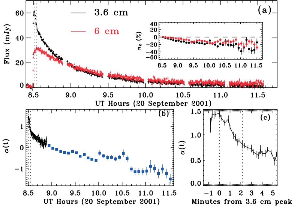
Fig. 15 A remarkable radio flare on the dm3.5e EV Lac from Osten et al (2005) with the spectral indices calculated from observations at the two observed frequencies. Reproduced with permission.
