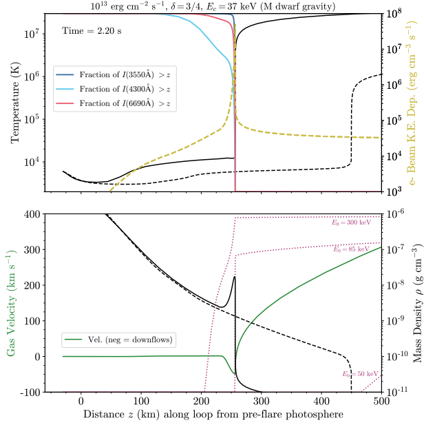
Fig. 21 RADYN model of the low flare atmosphere after 2.2 s of heating by a high-flux, F13 ( 10^{13} erg cm -2 s -1 ), double power-law electron beam (Kowalski et al, 2015). (top panel) The cumulative of the contribution function to the emergent intensity, I(\lambda = 3550\text{\AA}) , shows that the chromospheric condensation becomes optically thick in the Balmer continuum. The emergent blue-optical ( \lambda = 4300\text{\AA} ) continuum intensity has larger contribution from the layers below the condensation, which is the large increase in gas density in the bottom panel. (Bottom panel) Several trajectories of nonthermal electrons are shown on top of the gas dynamic quantities (the initial kinetic energies are indicated, and the kinetic energy variations, E(z) , are normalized from 0 to 1 on a linear scale). The initial temperatures and gas densities are shown as black dashed lines. A movie is available online.
