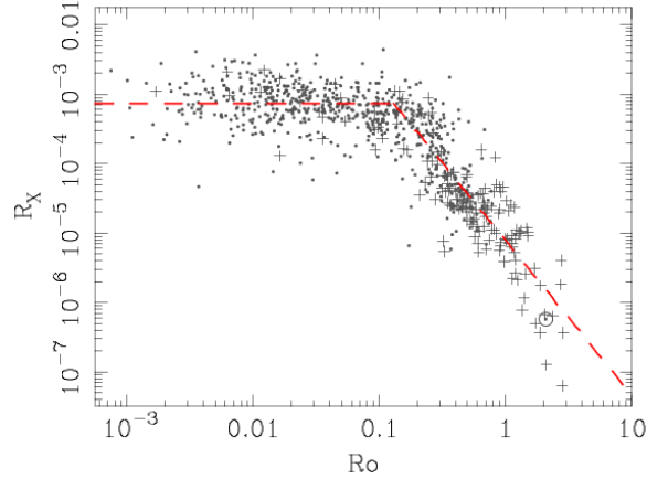
Fig. 4 Quiescent R_X = L_X/L_{\text{bol}} vs. the Rossby number for a large sample of stars, reproduced from Wright et al (2011) with permission. R_X is “saturated” at \approx 10^{-3} for stars with Rossby numbers \lesssim 0.1 , and R_X decreases according to a power-law for lower-activity stars.
