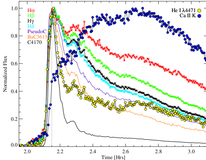
Fig. 9 Representative time-evolution of optical spectral quantities over a giant flare on the M4.5Ve star, YZ CMi. The peak optical broadband magnitude enhancements are listed in row (2) of Table 7. The emission line fluxes are integrated over wavelength, and all light curves are normalized to their respective peak fluxes. The C4170' light curve is a proxy for the flare-only blue continuum flux averaged over \lambda = 4155 - 4185 \text{ \AA} and is the fastest to decay after its peak flux is attained. The H \alpha and Ca II K emission lines are the slowest. Figure reproduced from Kowalski et al (2013) with permission.
