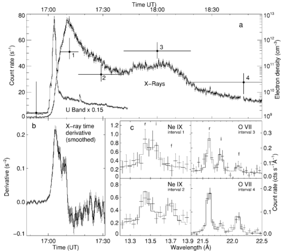
Fig. 18 A remarkable example of the Neupert effect in a stellar flare in Proxima Centauri; figure reproduced with permission, from Güdel et al (2002a). The U -band light curve is a (thermal) proxy for the nonthermal, impulsive energy deposition into the lower atmosphere. This flare was subsequently studied and modeled in Güdel et al (2004) and Reale et al (2004).
