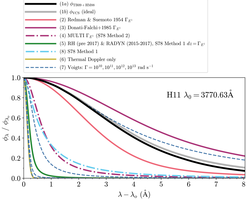
Fig. 28 A variety of approximations to opacity line profile functions for the Balmer series have been used in stellar flare modeling codes over many decades. This figure summarizes the differences in models of the line profile function, \phi_\lambda , for the H11 Balmer line (see also Johns-Krull et al, 1997 , for a similar figure for the H10 line). The calculations use n_e = n_p = 3.16 \times 10^{14} \text{ cm}^{-3} , or about 10x larger than in Fig. 27 , and thermal Doppler broadening at T = 10^4 \text{ K} is included. The “ideal” profiles, \phi_{VCS} , are the VCS73 calculations from Lemke (1997) , and do not account for line narrowing due to occupational probability / level dissolution. Several Voigt profiles are also plotted for a range of Lorentzian FWHM values, \Gamma . Currently, the most accurate theory corresponds to the \phi_{TB09+HM88} (solid black) curve.
