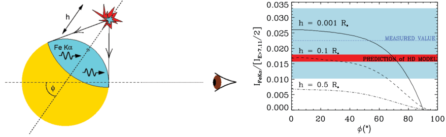
Fig. 32 Geometrical inference from spectral analysis of the 6.4 keV (1.94 Å) Fe K \alpha emission line during a flare on the giant star HR 9024, reproduced from Testa et al (2008) with permission. The X-rays from hot flare loops fluoresce the neutral iron in the surrounding photosphere. The modeling leverages hydrodynamic modeling from Testa et al (2007).
