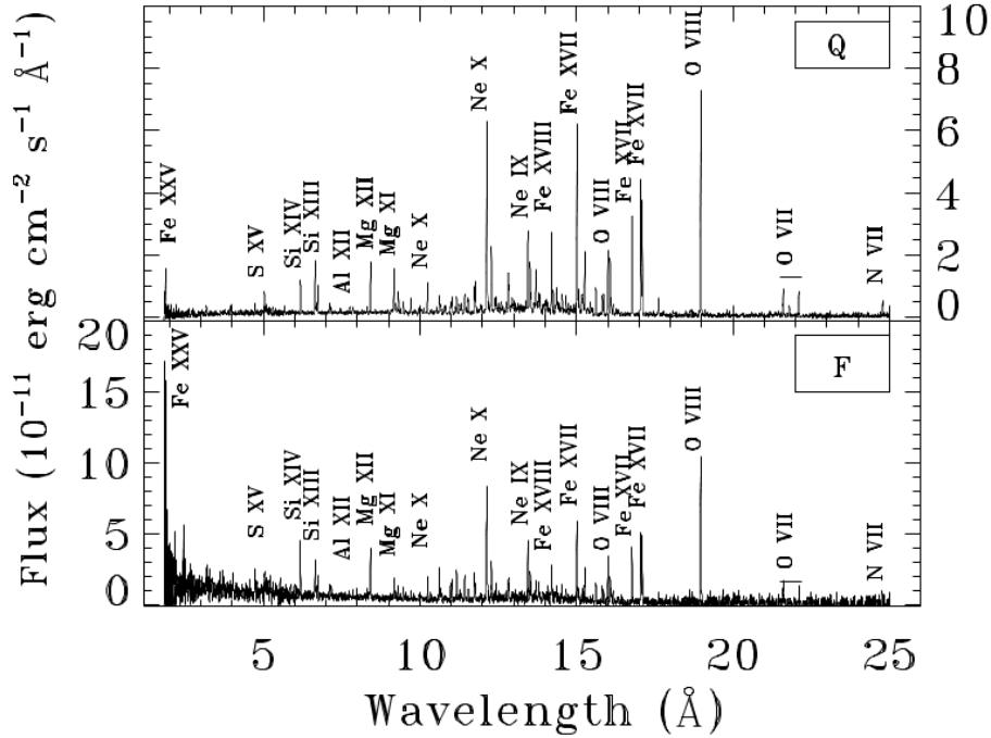
Fig. 17 X-ray spectra from Chandra during quiescence (top) and flaring (bottom) in the active binary \sigma^2 Coronae Borealis, reproduced from Osten et al (2003) with permission. The authors note the enhanced continuum flux increasing towards shorter wavelengths in the flare spectrum.
