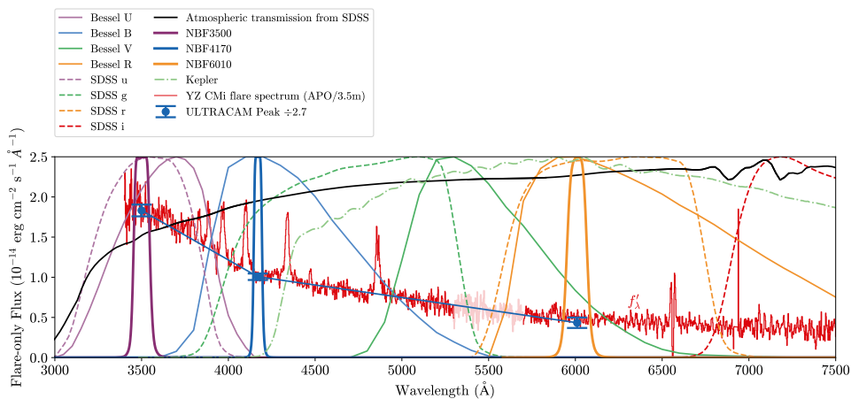
Fig. A1 Quantum efficiency curves of common optical filters, normalized to peak transmission. An example of a terrestrial atmospheric transmission curve from the Sloan Digital Sky Survey is shown for an airmass of 1.0 at the Apache Point Observatory. One should note that the quantum efficiency of the CCD, telescope primary mirror, and other optical elements are not included. For reference, the impulsive phase flare spectrum from the IF4 event in Kowalski et al (2016) is shown. The wavelengths that are affected by the dichroic are in a lighter shade of red. The ULTRACAM photometry (NBF3500, NBF4170, NBF6010) at the peak of this flare were calibrated independently, and they are scaled to account for the factor of ten shorter integration time. The flare data were obtained from the Zenodo repository at: https://doi.org/10.5281/zenodo.45878 .
