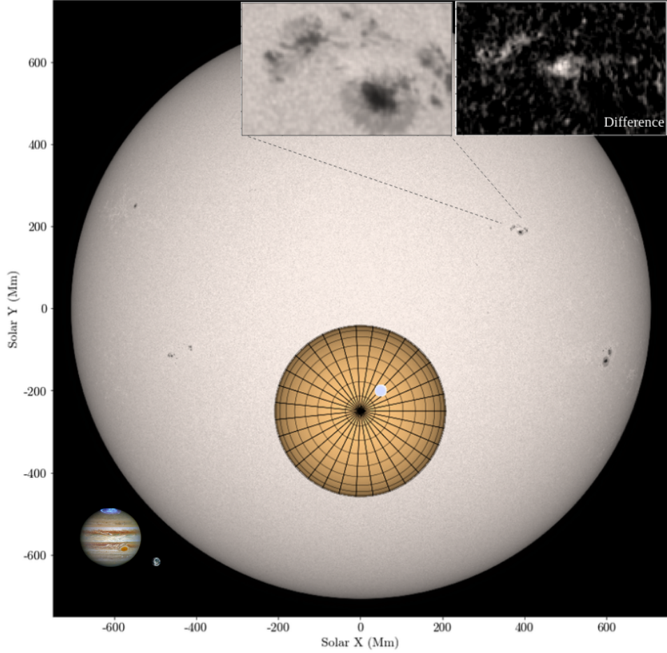
Fig. 31 Sizes to scale. An image of the Sun at \lambda = 6173 \text{ \AA} from the Helioseismic and Magnetic Imager (HMI; Scherrer et al, 2012) on SDO, a representative size of an active mid-type (MV3e-MV4.5e) M star ( R_{\text{star}} = 0.3R_{\text{Sun}} ), and a circular flare area ( \approx 5 \times 10^{18} \text{ cm}^2 ) that corresponds to about 0.5% of the visible hemisphere of this hypothetical M star. For comparison, Earth and Jupiter are shown to scale. The insets each have a field-of-view of \approx 10^{19} \text{ cm}^2 , and they show an image of the solar active region in the NW quadrant during the hard X-ray impulsive phase of the SOL2014-03-29T17:48 X1.0 flare (total intensity left, difference image right). For a detailed analysis of the HMI data of this solar flare, we refer the reader to Kleint et al (2016). Jupiter image credit: NASA, ESA, and J. Nichols; Earth image credit: GOES/NOAA/NESDIS.
