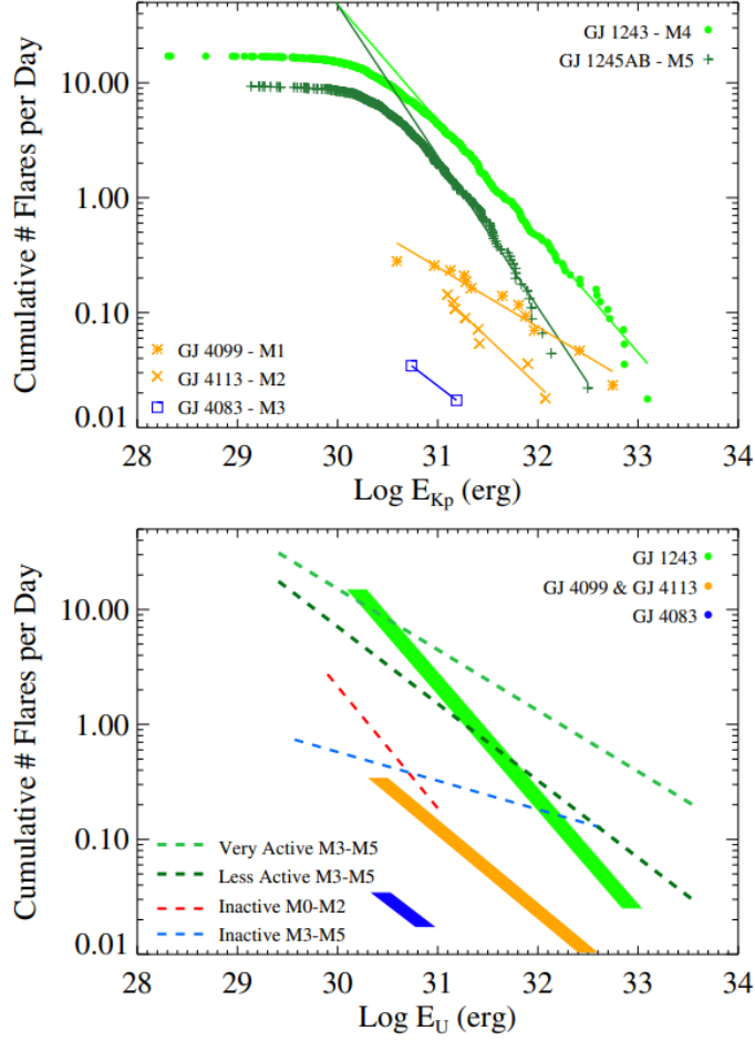
Fig. 7 Flare frequency distributions of several main-sequence M stars in the Kepler band (top) and in the U -band (bottom). Figure reproduced from Hawley et al (2014) with permission. Note the spread in flare rates in the bottom panel among the very active and less active stars of the same spectral types.
