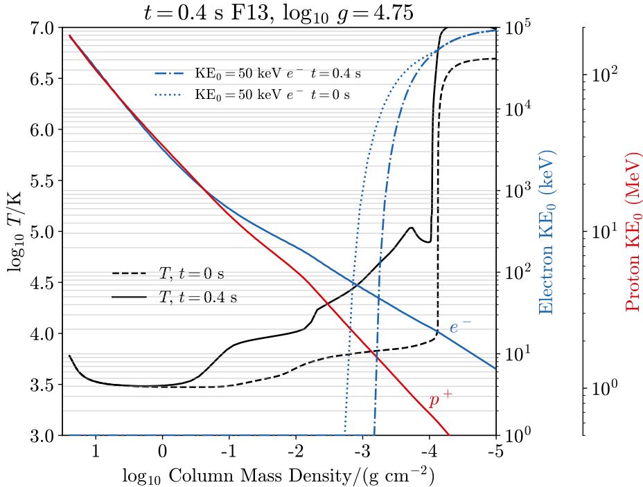
Fig. 24 A pre-flare and flare model (from the RADYN code) of the temperature distribution in the low atmosphere compared to Coulomb stopping depths of beam particles. For reference the (pre-flare) photosphere and upper photosphere corresponds to \log_{10} m_c > 1 on this plot ( m_c is the column mass density in units of \text{g cm}^{-2} ). The collisional stopping depths of mono-energetic beam particles are shown on the right using Equation 19. The kinetic energy decrease of an electron with injected energy of 50 keV is shown for each state of the atmosphere; these two curves are on a linear scale and normalized to 1.0 at the top of the loop (where they are injected) outside the range of the plot on the right. An electron gets stopped at higher altitudes when the chromosphere has experienced a large amount of hydrogen ionization; as the atmosphere further evolves, the lower energy electrons in the beam can be stopped in the evaporation flows ( cf. Fig. 21), and all the rest of the beam particles except for the highest energy electrons are stopped in the chromospheric condensation (Fig. 2(right)). Note, these “cold-target” stopping depth approximations for the protons are not accurate significantly below \lesssim 1 MeV at which the warm-target transport treatment becomes essential (Allred et al, 2020).
