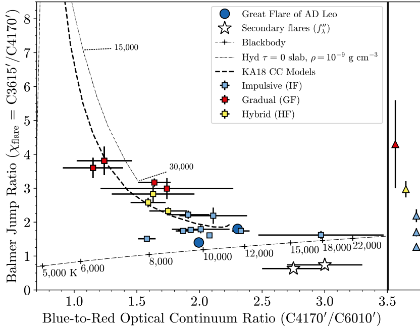
Fig. 12 Compilation of impulsive-phase continuum flux ratios (color-color diagrams) from spectra (Kowalski et al, 2013, 2016, 2019b). The y-axis is a measure of the Balmer jump ratio, and the flux ratios on the x-axis correspond to optical color temperatures. Note that the x and y uncertainties are correlated, but only marginal error bars are shown. The prime symbols indicate that a pre-flare flux has been subtracted. The optical continuum colors from the Great Flare of AD Leo (Hawley and Pettersen, 1991) are estimated from extrapolations of blackbody curve fits over the \lambda = 3800 - 4440 Å range (Kowalski et al, 2013). The wavelength range of C4170' can be seen in the right panel of Fig. 11. The flux ratio values at the peaks of flares indicate optical depths between blackbody radiation and optically thin hydrogen recombination radiation. The general trend is well-reproduced by approximations (KA18 CC models; Kowalski and Allred, 2018) to the dynamic atmospheres in RHD simulations (Sect. 8.2). In the right margin plot, flares with Balmer jump measurements only are shown. The flares are color-coded to their U -band impulsiveness (IF/HF/GF) classification. Other flare-peak flux ratios from narrowband ULTRACAM photometry (Kowalski et al, 2016) are summarized in Appendix B. The color temperatures corresponding to the blue-to-red flux ratios in this figure are typically \gtrsim 1500 K less than that obtained from spectral fitting over the \lambda = 4000 - 4800 Å range. All data in this figure are provided in supplementary online material hosted on Zenodo.
