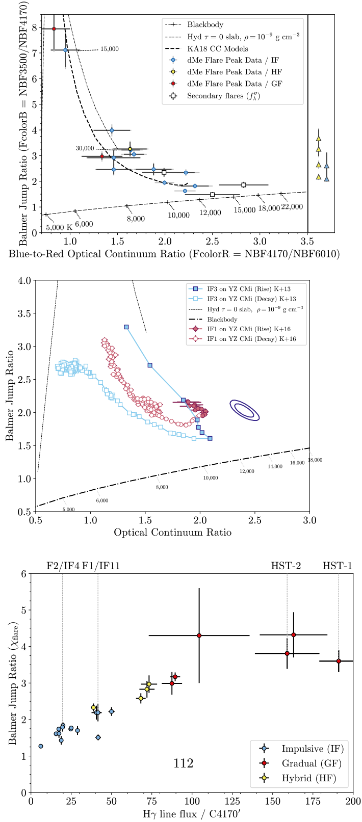
Fig. B2 ( Top ) Flare-peak colors from ULTRACAM narrowband filter ratios; similar to Fig. 12 and see text for details. ( Middle ) Evolution of flare colors in two large flares on YZ CMi. Time increases over the tracks in a clockwise direction. These data have small statistical uncertainties (which are shown) but non-negligible systematic errors. The uncertainties are correlated, which we show for representative 5% systematic absolute color calibration uncertainties in both flare colors located at (x, y) \approx (2, 2) . The error-ellipses indicate representative joint probabilities: the outer is the joint 68% confidence interval, while the inner translates to the marginal 68% uncertainties. ( Bottom ) Flare-only, line-to-continuum flux ratios from the same peak spectra in Fig. 12 in the main text.
