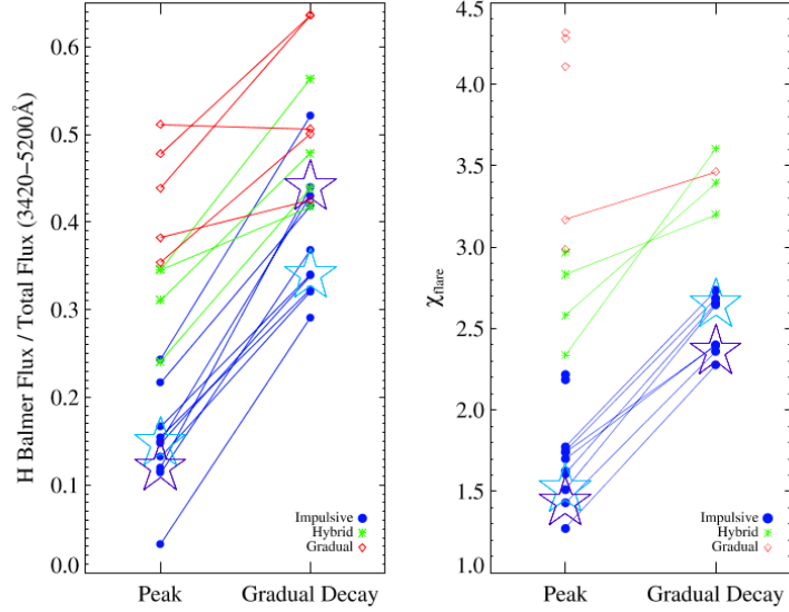
Fig. 13 Energy of the hydrogen Balmer component vs. the optical continuum energy evolution in a large sample of MVe flares (reproduced from Kowalski et al 2013 with permission). The Balmer jump ratios ( \chi_{\text{flare}} ) increase into the gradual decay phase and are also generally correlated with the IF/HF/GF classification scheme. The hydrogen Balmer component includes an estimate for the Balmer continuum flux above an optical continuum model extrapolation to \lambda < 3650 \text{ \AA} . Several more flares with comparable spectroscopy (Kowalski et al, 2016, 2019b) since this result have been consistent with these trends.
