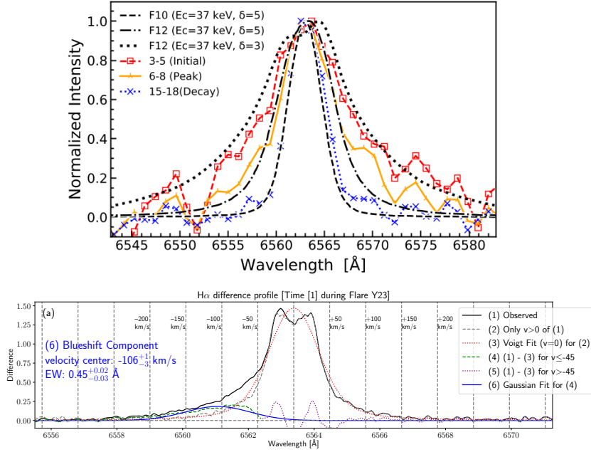
Fig. 22 (Top) Model spectra of H \alpha that were calculated with the RADYN code and analyzed in Namekata et al (2020). The larger electron beam heating rates reproduce the broad, symmetric Balmer lines in an AD Leo flare. Figure reproduced with permission from Namekata et al (2020). (Bottom) Echelle resolving power, flare-only spectra of the H \alpha line during the decay of a large flare on YZ CMi. This figure demonstrates the phenomenological Voigt profile + Gaussian modeling that is used to isolate and characterize the asymmetries in the wings of the Balmer lines. In this spectrum, a Gaussian model is fit to the broad blue asymmetry; reproduced from Fig. 42(a) in Notsu et al (2023), with permission.
