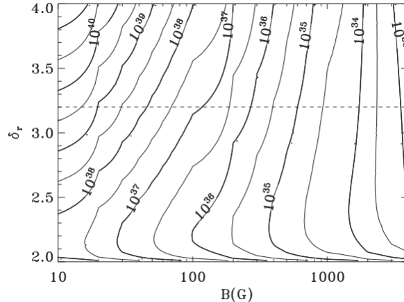
Fig. 29 A range of possible nonthermal electron beam power-law indices and magnetic field strengths that can be constrained from gyrosynchrotron data of stellar flares; reproduced from Figure 6 in Osten et al (2016) with permission. See also Smith et al (2005) and MacGregor et al (2021) . Contours of constant electron beam kinetic energies add a third constraint. Cross sectional footpoint areas from optical data can constrain the beam flux density for forward modeling inputs ( Osten et al, 2010, 2016 ).
