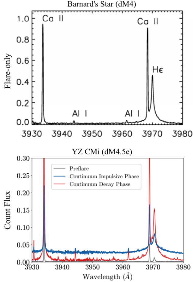
Fig. 26 Dramatic broadening differences between hydrogen and metallic emission lines, such as the Ca II resonance lines, in flare spectra are considered evidence for the important role of pressure broadening of hydrogen. The pressure broadening of hydrogen constrains the charge densities (and optical depths) in the flare chromosphere. This conclusion is supported by detailed spectral synthesis with, e.g., the RADYN, RH, MULTI codes. The top figure shows these effects during a flare on the dM4 star Gl 699, reproduced from Paulson et al (2006), and the bottom panel shows the coarse temporal evolution of the broadening differences during a flare (Vida et al, 2019) on the dM4.5e star YZ CMi.
