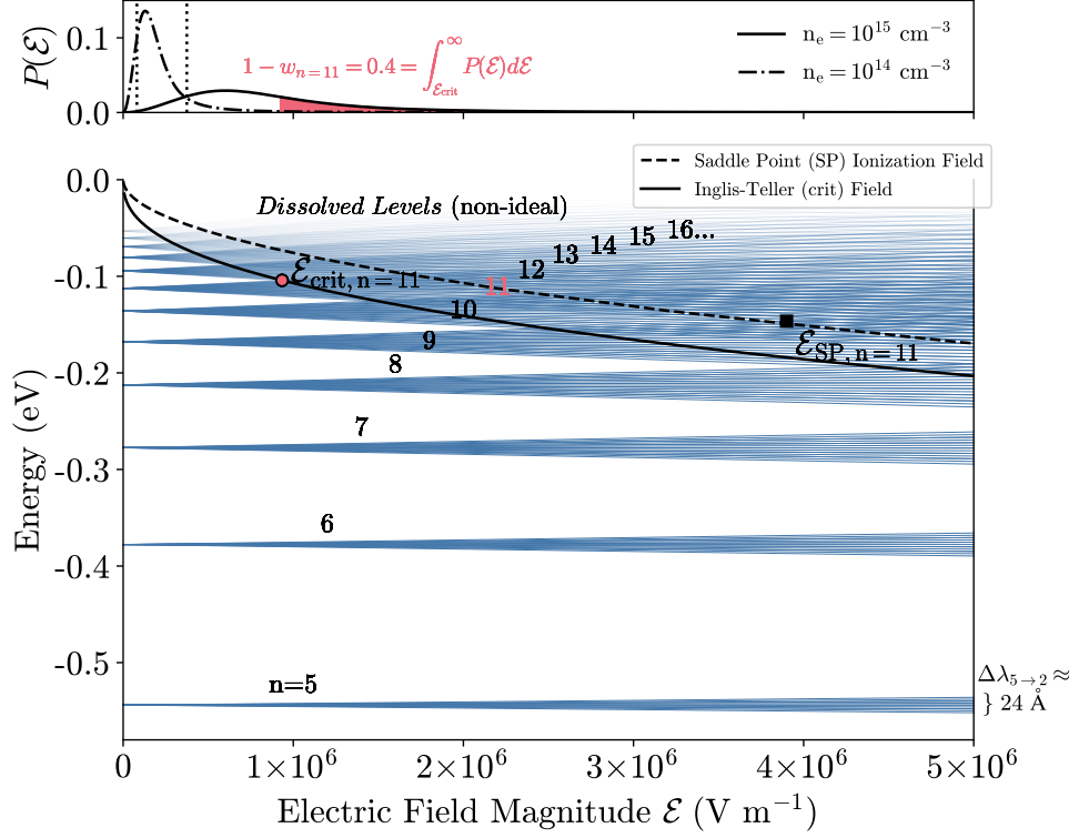
Fig. D8 Energy level splitting for hydrogen in a static external electric field as a function of the electric field (in SI units). A principal level n is split into roughly 2n - 1 (including the unshifted) sub-states. For even n , there is an unshifted component. Every split sub-state ( k_1, k_2, m ) is a mix of all the l -states for that value of n . The maximum splitting of the n = 5 level shown here corresponds to 0.016 eV, which would correspond to a maximum wavelength displacement of \Delta\lambda \approx 24 \text{ \AA} for the H\gamma transition. Only levels that can result in a dipole transition with n = 2 have been plotted. The transitions with \Delta m = 0 are known as the \pi components, and \Delta m \pm 1 are the \sigma components. The field strength that forms a “saddle point” (potential energy maximum) and destroys all levels > n in hydrogen is shown as a function of n (if there is a saddle-point in the potential, then tunneling is allowed as well; Bethe and Salpeter, 1957 ). The field ionization of hydrogen has been observed (see the photograph from Rausch v. Traubenberg et al (1930) that is reproduced in Montgomery et al 2022 ). The Inglis-Teller relation corresponds to the critical field that causes the “bluest” sub-state of n to intersect with the “reddest” sub-state of n + 1 , which occurs at a much smaller electric field for a given n than the saddle point estimate (the ratio of the critical field to the saddle-point field is given by the factor known as K_n in the literature). Holtsmark probability distributions of electric field magnitudes are shown in the top panel to illustrate an occupational probability ( w_n ) calculation for n = 11 and n_e = 10^{15} \text{ cm}^{-3} . A “normal field”, F_0 , is the electric field magnitude at an average interparticle separation; the critical fields for n_e = 10^{14} and 10^{15} \text{ cm}^{-3} are indicated by vertical dotted lines in the top panel.
