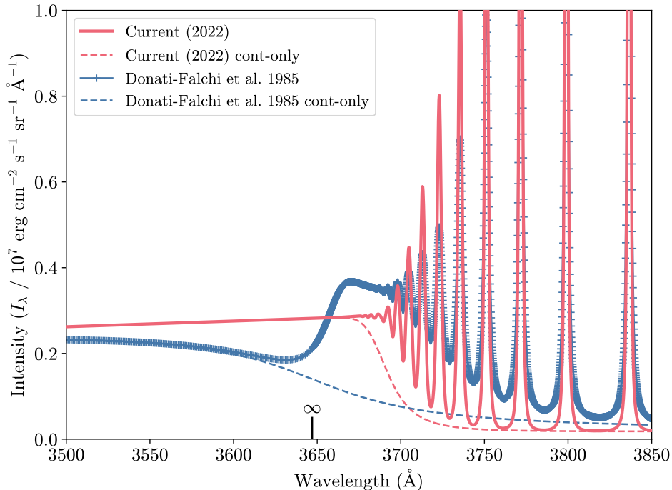
Fig. 27 Direct comparisons of two methods (Donati-Falchi et al, 1985; Kowalski et al, 2017b) for calculating the Balmer jump spectral region in solar and stellar flares. The emergent LTE intensity is calculated from a slab with n_e = 3.9 \times 10^{13} \text{ cm}^{-3} . The method from Donati-Falchi et al (1985) predicts a “blue continuum bump”, whereas the current treatment with occupational probabilities predicts an extension of the Balmer continuum intensity to wavelengths longward of the “ideal” recombination limit (indicated by an \infty symbol) at \lambda = 3646 \text{ \AA} .
