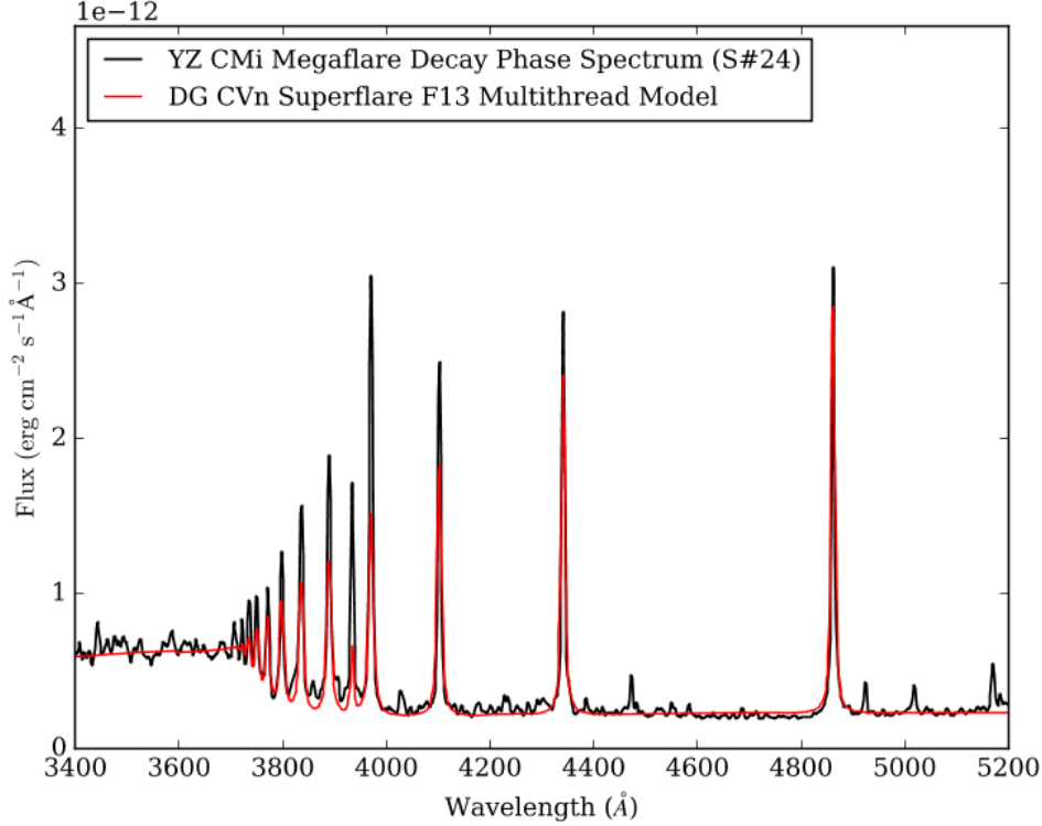
Fig. 30 Gradual-decay phase, flare-only spectrum of a megaflare on the MV4.5e star YZ CMi (Kowalski et al, 2010). Multi-thread RHD modeling of another superflare on DG CVn (Osten et al, 2016) adequately reproduces the Balmer jump, optical continuum shape, and some of the hydrogen Balmer emission line properties (but some important shortcomings remain). Each RHD model component is calculated self-consistently, but the linear superposition of the model components is semi-empirical; see discussion in Kowalski et al (2017b) and Kowalski et al (2019a).
