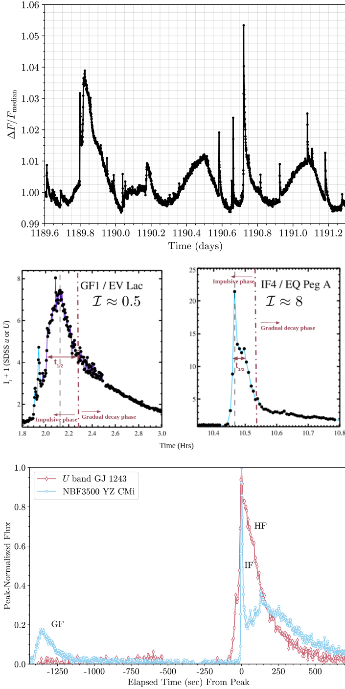
Fig. 8 Representative high-cadence optical light curves of M Ve flares. (Top) A randomly chosen section of the 1-minute cadence Kepler light curve of GJ 1243 from Davenport et al (2014) showing a variety of classical and complex flares superimposed on the modulation, which is due to starspots (Davenport et al, 2015). The data were obtained from https://github.com/jradavenport/GJ1243-Flares . Note, there was a single flare event (not shown) that was observed simultaneously in both Kepler and in the U -band (Hawley et al, 2014). For reference, this flare had a relative peak contrast of \Delta F/F_{\text{median}} = 0.014 in the Kepler band, a peak contrast of I_f = 0.9 in the U band, and a total U -band energy of 10^{31} erg. (Middle left) The impulsive and gradual decay phases of a high-energy gradual flare (GF) event on EV Lac; reproduced with permission from Kowalski et al (2013). The impulsive phase and gradual decay phases are indicated. At the peak (vertical black dashed line), GF-type events like this one have large Balmer jumps, which are still much smaller than predicted by optically thin hydrogen recombination theory alone (e.g., Sect. 7.2.1). The t_{1/2} = 13 min is the FWHM of the light curve, and the U -band impulsiveness index, \mathcal{I} = I_f/t_{1/2} , is 0.5 for this flare. (Middle right) An example high-energy IF event ( t_{1/2} = 2.5 min, \mathcal{I} = 8.3 ) on EQ Peg A, reproduced with permission from Kowalski et al (2013). (Bottom) Examples of lower energy flares within the flare IF/HF/GF classification scheme based on the impulsiveness in the U -band or a narrow-band filter (NBF) with \lambda_c = 3500\text{\AA} . The HF and IF events have similar peak contrasts ( I_f = 2.7 - 3.7 ) but differ significantly in the values of t_{1/2} (14 s and 120 s). The IF and GF events are referred to as IF4 and GF2 in Kowalski et al (2016); the HF event is referred to as the HST-2 flare in Kowalski et al (2019b). Note, the flare-only impulsive-phase spectrum of the IF event is shown in comparison to common photometry filters in Appendix A.
