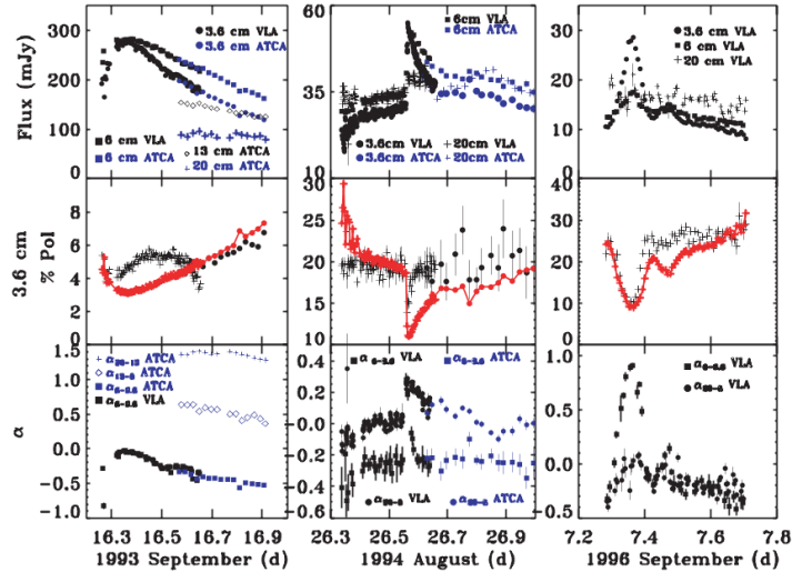
Fig. 16 Flux (top row), polarization (middle row), and spectral indices (bottom row) during three gyrosynchrotron radio flares from the RS CVn HR 1099, reproduced from Osten et al (2004) with permission.
