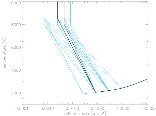
Fig. 20 Demonstration of semi-empirical temperature adjustments used to model the red- and blue-wavelength optical spectra of a giant flare from CN Leo. Figure from Fuhrmeister et al (2010) reproduced with permission from the author. See also Fuhrmeister et al (2011) and Fuhrmeister et al (2005) for similar approaches for modeling flares from Proxima Centauri and the dM6 star AZ Cnc, respectively.
