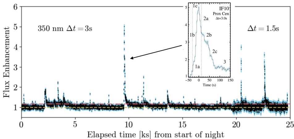
Fig. 1 A light curve of Proxima Centauri in a narrowband (filter FWHM of 100 \text{ \AA} ) centered in the near-ultraviolet, U -band wavelength regime. These data are from Kowalski et al (2016) and can be obtained from the Zenodo repository at https://doi.org/10.5281/zenodo.45878 . The horizontal dashed lines indicate the mean flux enhancement (1.0) and 3\sigma above the mean (where \sigma is the standard deviation outside of flaring). The inset shows the flare peaking at 2010 May 25 01:31:02 UT, which is referred to as the “IF10” event in Kowalski et al (2016). The inset shows time relative to peak.
