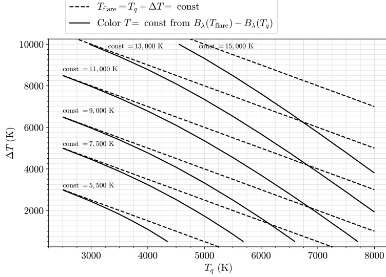
Fig. C4 Lines of constant blackbody flare temperatures ( T_{\text{flare}} ) and lines of constant blackbody color temperatures that are calculated after subtracting a quiescent blackbody surface flux spectrum, S_{\lambda,q} = B_{\lambda}(T_q) , from the flare model spectrum, S_{\lambda,\text{flare}} = B_{\lambda}(T_{\text{flare}}) . The color temperature calculations, here shown for \lambda_1 = 4170 \text{ \AA} and \lambda_2 = 6010 \text{ \AA} , from stellar flare data usually account for or consider these issues in M dwarf flares (Hawley et al, 1995; Kowalski et al, 2016), but hotter flare color temperatures in higher-mass stars could be a result of “oversubtraction” effects.
