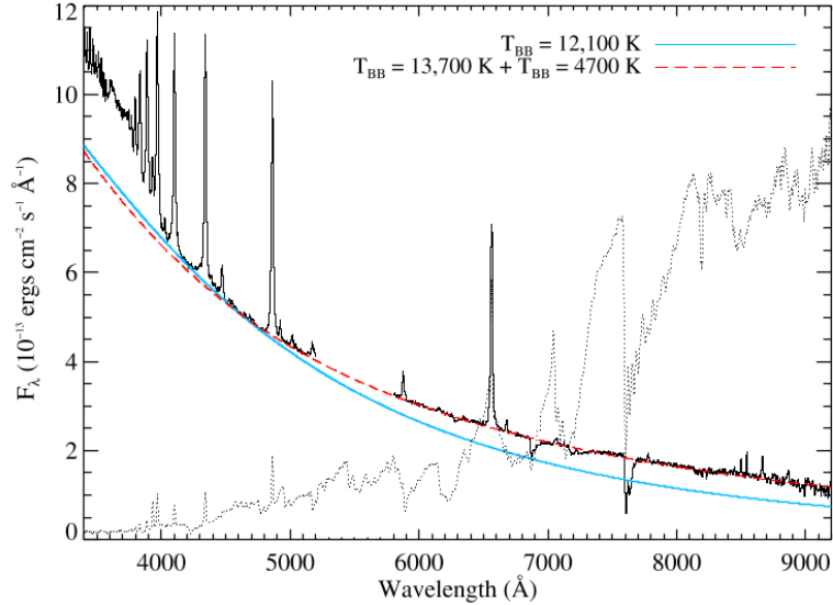
Fig. 10 Flare spectrum at the peak of the large, impulsive-type (IF) event on YZ CMi in Fig. 9. Several blackbody fits to optical ( \lambda \geq 4000 Å) continuum regions are shown. The flare spectrum (black) has the pre-flare (dotted) spectrum subtracted. Figure reproduced from Kowalski et al (2013) with permission.
