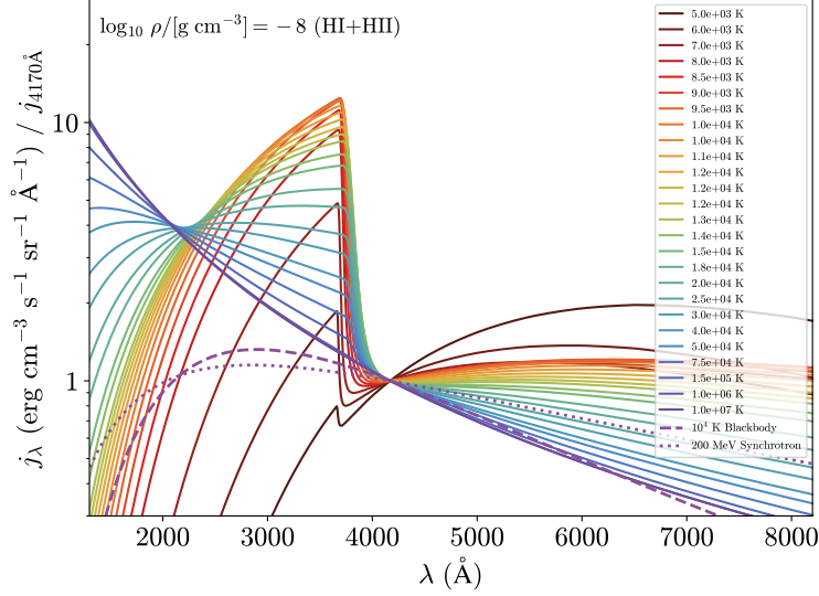
Fig. C5 Hydrogen LTE emissivity calculations with bound-free (recombination) emissivity from H I and H - and free-free (thermal bremsstrahlung) emissivity from H II. The spectral shapes here are identical to the shapes of intensity spectra, I_\lambda , that emerge from optically thin, homogeneous slabs. A blackbody function and a mono-energetic synchrotron spectrum is shown for comparison. The smooth transitions from the Balmer jump to the optical wavelengths are caused by the “dissolved level Balmer continuum” (Dappen et al, 1987), which extends to redder wavelengths for larger electron densities.
