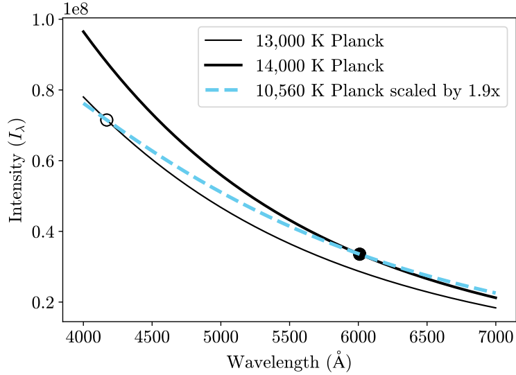
Fig. C3 Demonstration showing the relationship between a color temperature and wavelength-dependent radiation (brightness) temperatures at \lambda = 4170 \text{ \AA} and \lambda = 6010 \text{ \AA} .
