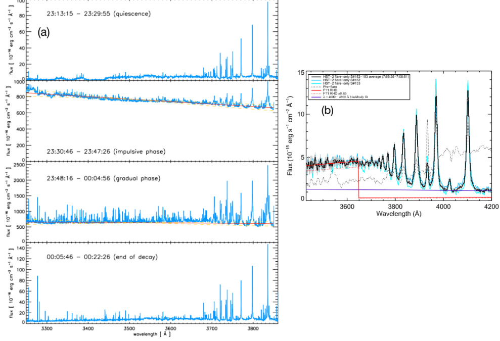
Fig. 11 (a) VLT/UVES echelle ( R \sim 40,000 ) spectral observations at \lambda < 3860 \text{ \AA} that nearly extend to the terrestrial atmospheric cutoff. These spectra show the evolution of a giant white-light flare on the M6Ve star CN Leo, reproduced from Fuhrmeister et al (2008) with permission. A T \sim 11,300 \text{ K} blackbody is fit in the impulsive phase (2nd from top), and the gradual phase spectrum is fit with a T \sim 9100 \text{ K} blackbody in the third panel. A catalog of the emission lines in the spectrum in the middle panel, extending to \lambda = 3060 \text{ \AA} , is available through VizierR. (b) Other MVe flares in the impulsive phase show a large Balmer jump and a flatter U -band continuum spectrum that decreases into the NUV at shorter wavelengths than shown here ( Kowalski et al, 2019b ) are not satisfactorily explained by a T \approx 9000 \text{ K} blackbody fit to the blue-optical continuum wavelengths. Here, the two blue-colored spectra correspond to the rise/peak phase and early gradual decay phase, respectively, which are averaged into the black spectrum. The red-colored spectrum is an optically thin hydrogen recombination continuum model from a RHD simulation that invokes a solar-type electron beam heating function; the model is scaled to the observed spectrum at \lambda \approx 3615 \text{ \AA} . The spectra have a low-resolving power, R \approx 600 , which is clearly sufficient for robust wavelength-integrated emission line fluxes. Figure reproduced with permission from Kowalski et al (2019b) .
