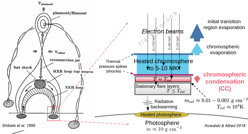
Fig. 2 (Left) Illustration of several salient features and processes in the standard model of solar flares, reproduced from Shibata et al (1995) with permission. (Right) Generalization of the chromospheric evaporation and condensation phenomena in radiative-hydrodynamic models of high-flux electron-beam heating at the footpoints of newly-reconnected flare loops (adapted from Kowalski and Allred, 2018). Here, we also include an illustration of the radiative backwarming of the photosphere, which is predicted by some 1D models (Allred et al, 2006) of flare chromospheres that are optically thin at Balmer and Paschen continuum wavelengths (see Fisher et al, 2012, for the expected geometry of 3D radiative backwarming of the photosphere).
