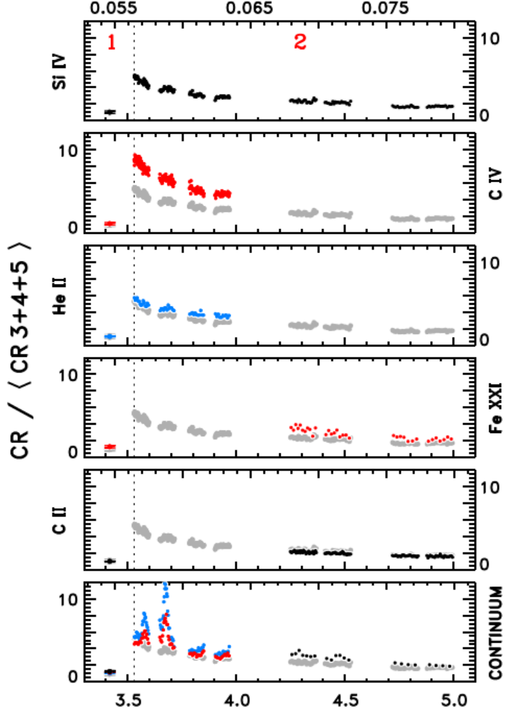
Fig. 14 Figure 7 from Ayres (2015b) , reproduced with permission, showing various FUV spectral quantities from HST/COS spectra during the decay phase of a large flare on the young solar analog, EK Dra. The bottom x -axis is elapsed time (hr) and top x -axis is rotational phase. Note the bursts that only occur in the FUV continuum ( \lambda = 1435 \pm 25 \text{ \AA} , 1610 \pm 25 \text{ \AA} ). Later in the decay phase, shorter FUV wavelengths were observed by HST/COS, providing constraints on the continuum at \lambda = 1344.5 \pm 6 \text{ \AA} and \lambda = 1381.0 \pm 8.0 \text{ \AA} , the forbidden coronal line [Fe XXI] \lambda 1354 ( T_{\text{form}} \approx 10^7 \text{ K} ), and C II \lambda 1335.
