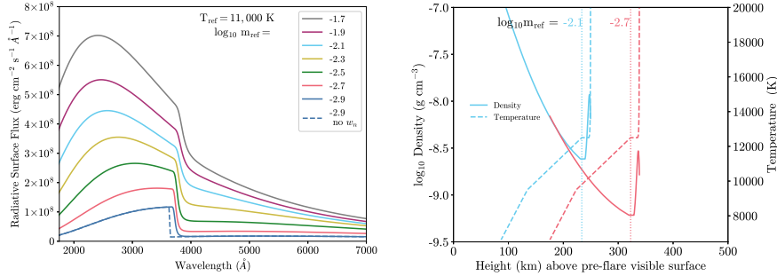
Fig. C7 (Left) LTE continuum flux spectra calculated from the parameterized evolution of chromospheric condensations from RHD models. (Right) Examples of two of the parameterized atmospheres.
